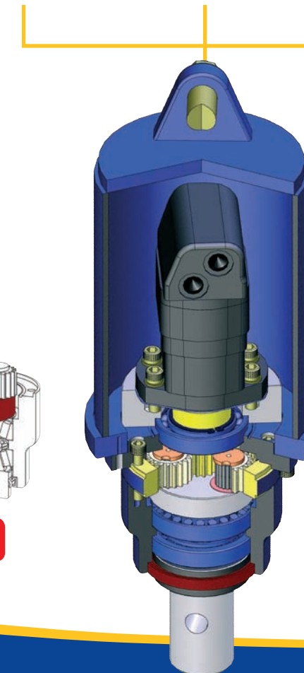
Cut away view of 3000 MAX Earth Drill
